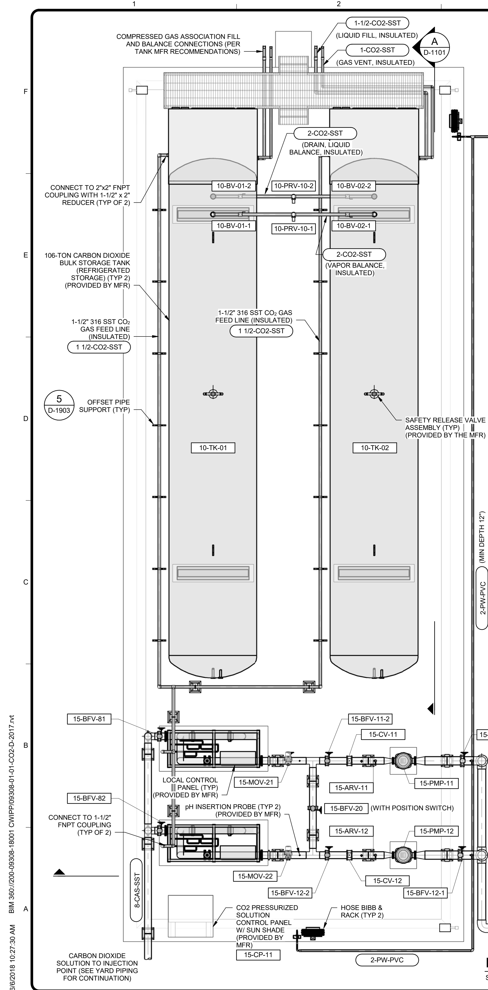
EQUIPMENT PLAN SCALE: 3/16" = 1'-0"
